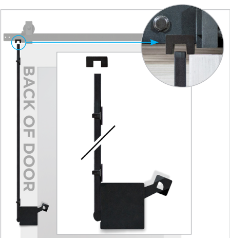
EASY LATCH HARDWARE (Barn Door privacy locking mechanism) BDF8000-MB
